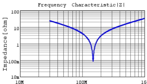
RCE5C2J221J1M1H03A |Z| DCOV, 25degC
