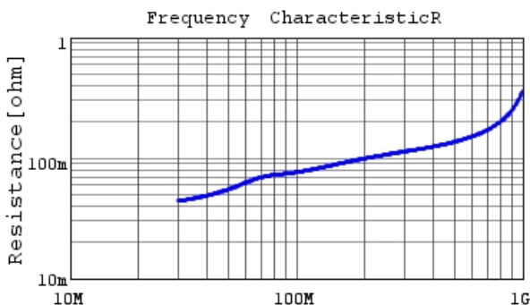
RCE5C2J221J1M1H03A R DCOV, 25degC
