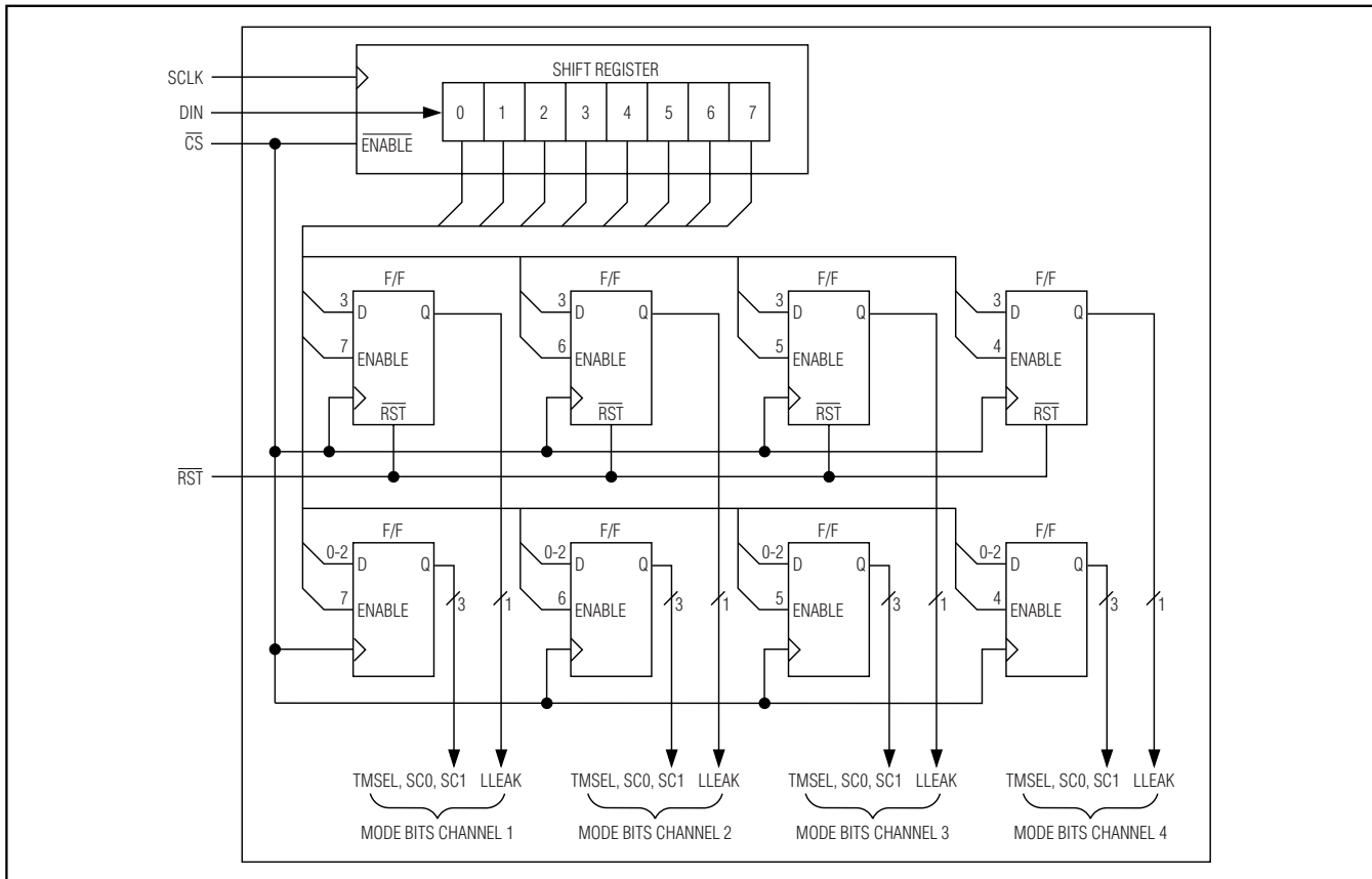
Figure 6. Serial Interface
