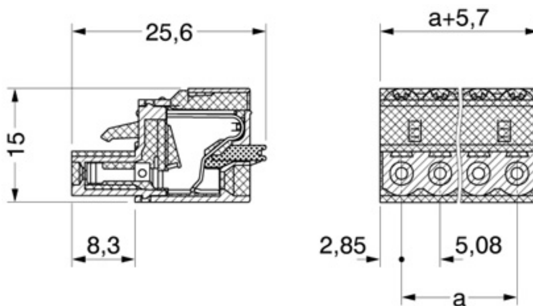
Dimensioned drawing
