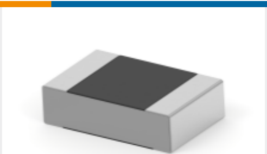
TE Part #2176238-7 CPF A 0805 22R 0.1% 25PPM 5K RL
