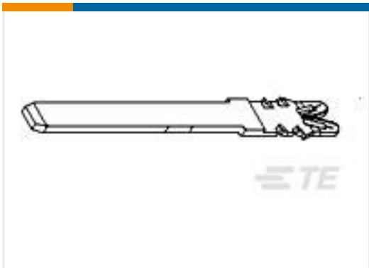
TE Part #1601112-2 131-187-014=TAB,110X032,STD SMZ
