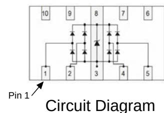
DFN2510-10L (DFN2510D-10))
