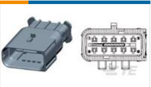
TE Part # 1801606-2 TAB HOUSING, MCON, 10 W, SEALED
