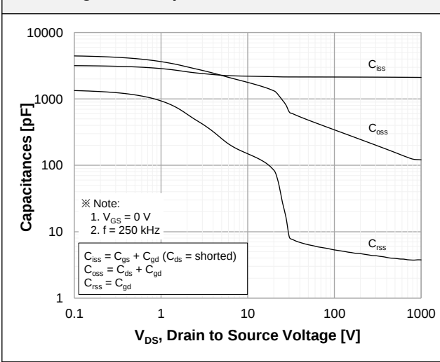
Figure 12. Capacitance Characteristics
