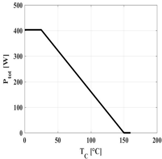
Figure 3: Power Dissipation
