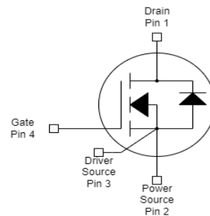
Figure 1 Symbol of SRC65R042B
