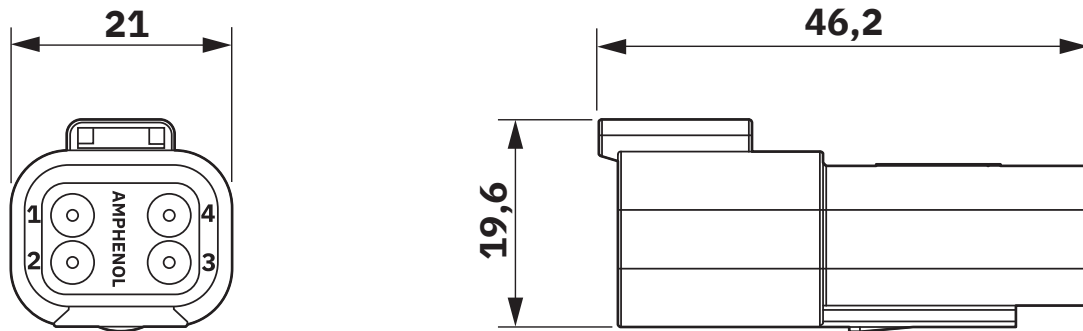
AT04-4P top view and side view
