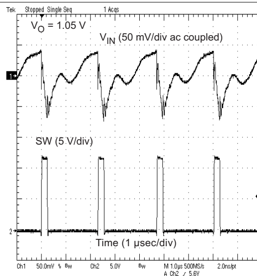
Figure 16. Input Voltage Ripple, I_{OUT} = 8\text{ A}
