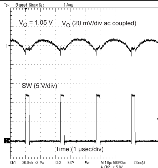
Figure 14. Output Voltage Ripple, I_{OUT} = 8\text{ A}
