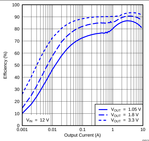
Figure 13. Light Load Efficiency
