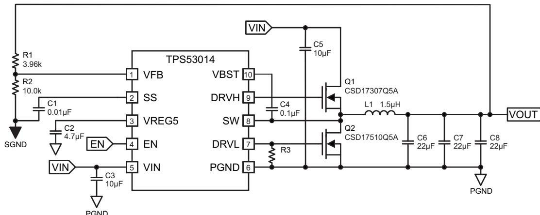
Figure 18. Application Schematic
