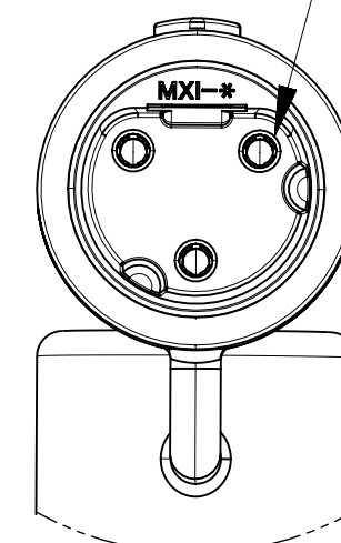
VIEW SHOWING KEYING OF 3 CIRCUIT VERSION
