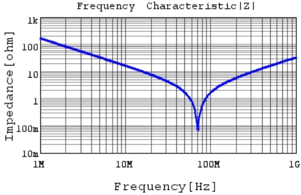
RCE5C2E102J1K1H03B |Z| DCOV, 25degC
