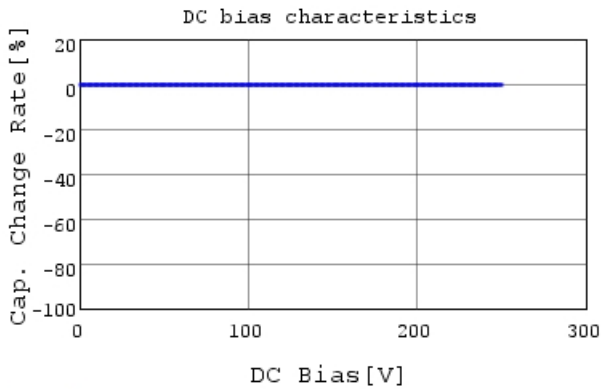
RCE5C2E102J1K1H03B C-DC bias capchange, 25.0
