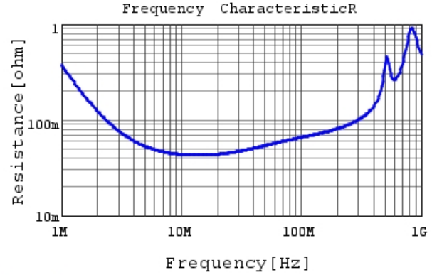
RCE5C2E102J1K1H03B R DCOV, 25degC
