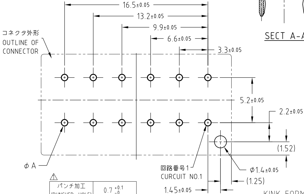
PCB.LAYOUT ON RECOMMENDATION
