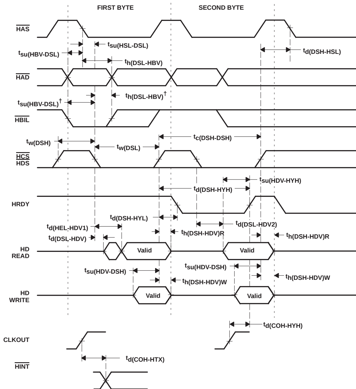
Figure 31. Read/Write Access Timing With \text{HRDY}
