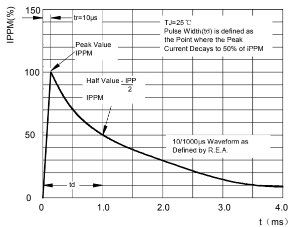
FIG3: Pulse Waveform
