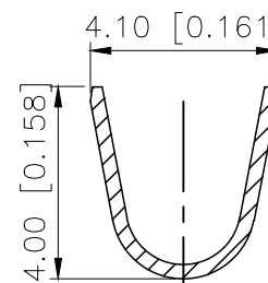
SECTION:B-B SCALE:1:1
