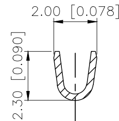
SECTION:A-A SCALE:1:1
