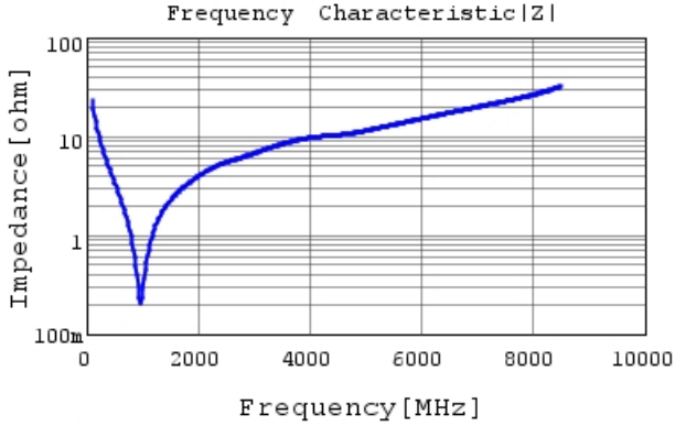
GRT1555C1E680JA02 |Z| DCOV,25degC
