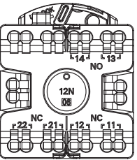
Three contacts (2NC + 1NO)
