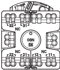
Three contacts (3NC)
