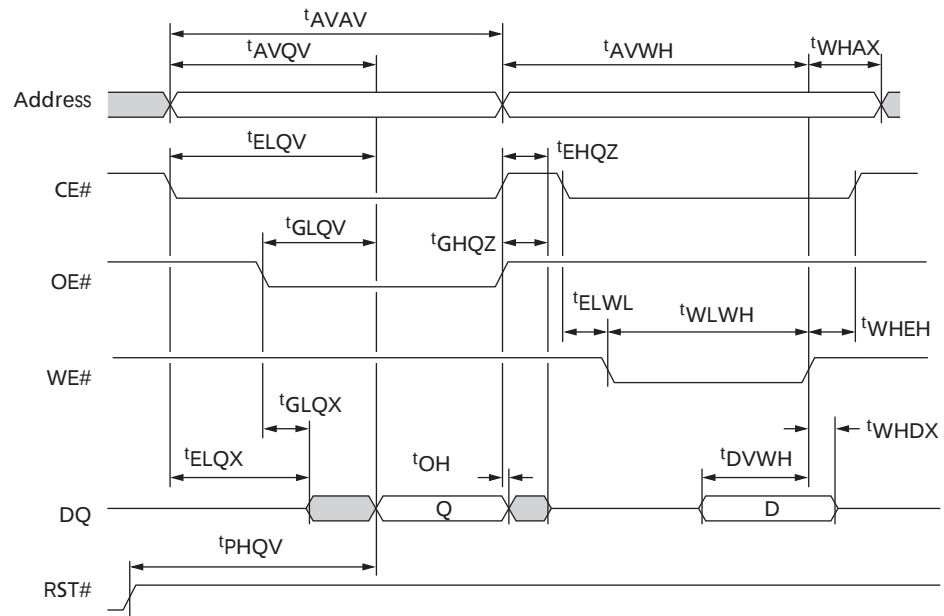
Figure 24: Asynchronous Read to Write Timing
