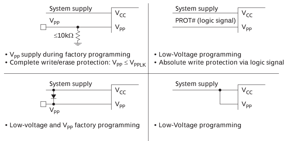
Figure 5: Example V_{PP} Power Supply Configuration
