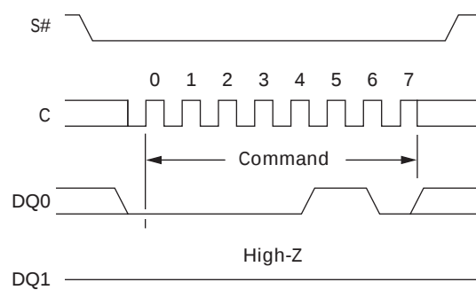
Figure 9: WRITE ENABLE (WREN) Instruction Sequence
