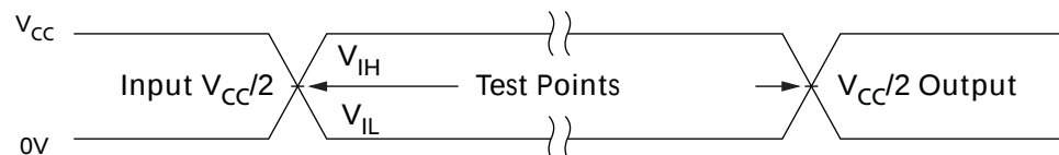
Figure 19: AC Input/Output Reference Waveform
