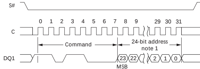
Figure 17: SECTOR ERASE (SE) Instruction Sequence
