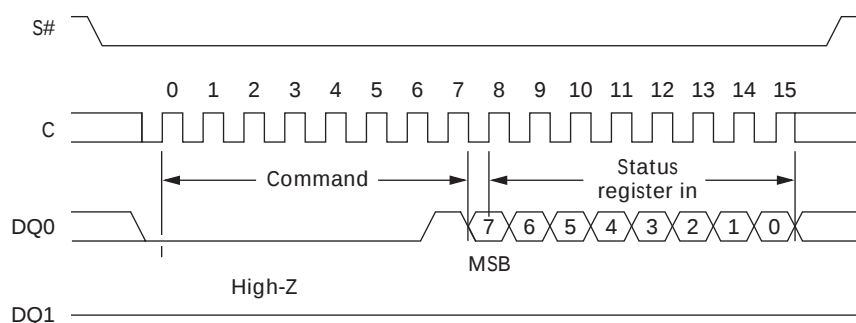
Figure 13: WRITE STATUS REGISTER (WRSR) Instruction Sequence
