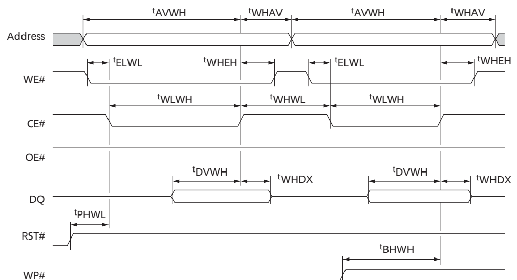
Figure 23: Write-to-Write Timing
