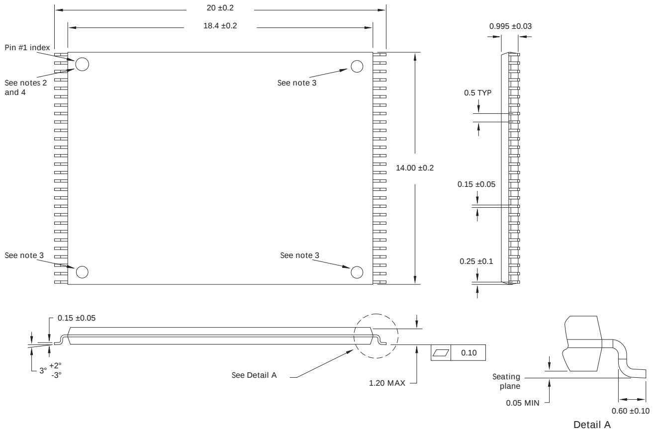
Figure 1: 56-Lead TSOP
