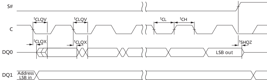
Figure 29: Output Timing
