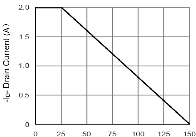
Figure 4 Drain Current
