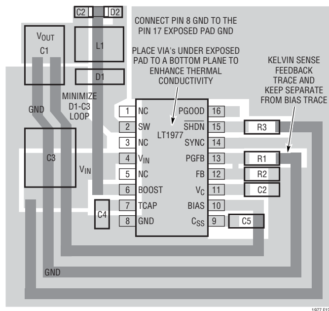
Figure 12. Suggested Layout
