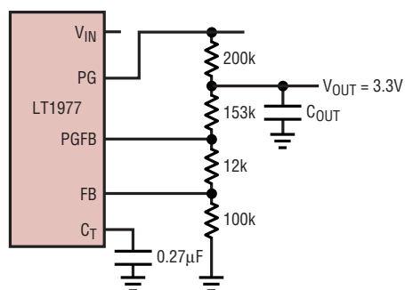
V_{OUT} Disconnect at 80% V_{OUT} with 100ms Delay
