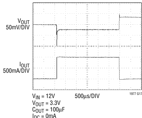
No Load 1A Step Response
