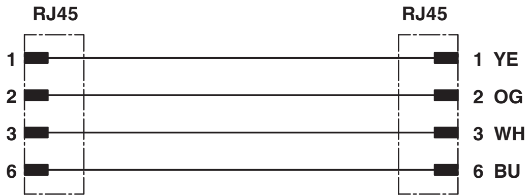
Circuit diagram
