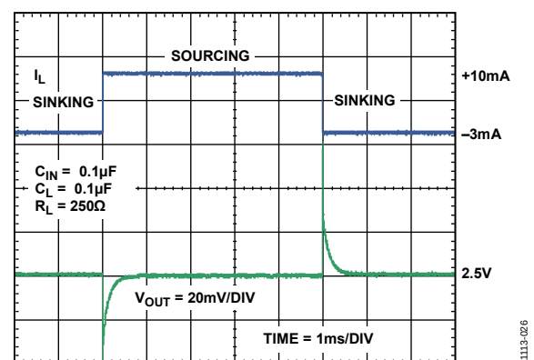
Figure 26. ADR3525 Load Transient Response
