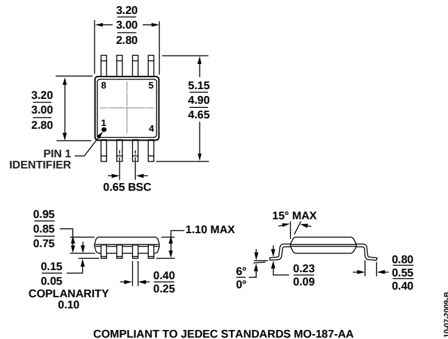
Figure 42. 8-Lead Mini Small Outline Package [MSOP] (RM-8) Dimensions show in millimeters
