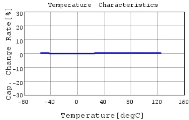
GRM0115C1E5R6WE01 C-Temp. capchange, DCOV, 1
