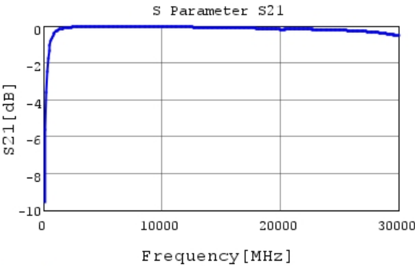
GRM0115C1E5R6WE01 S21 DCOV, 25degC
