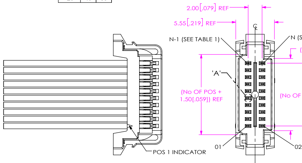
DETAIL 'B' SCALE 8:1
