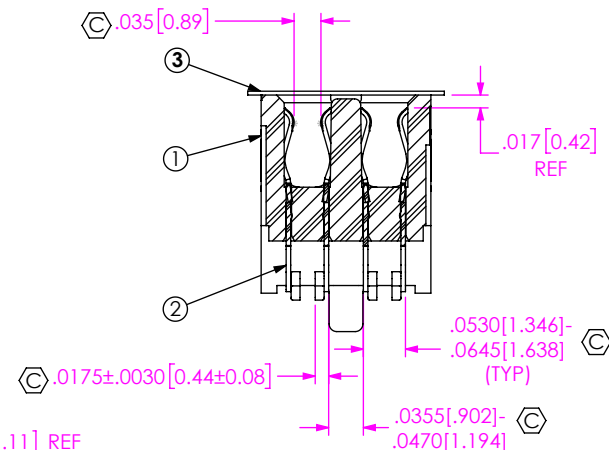
SECTION "A"-"A" SCALE 4 : 1
