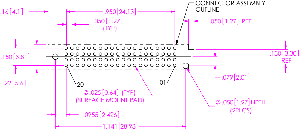
RECOMMENDED PCB LAYOUT SCALE 2:1
