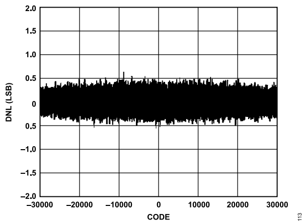
Figure 13. DNL
