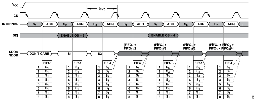
Figure 30. Rolling Average Oversampling Mode Configuration
