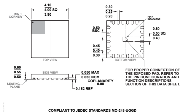
Figure 42. 24-Lead Lead Frame Chip Scale Package [LFCSP] 4 mm × 4 mm Body and 0.55 mm Package Height (CP-24-25) Dimensions shown in millimeters
