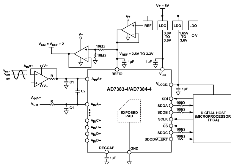
Figure 28. Typical Applications Circuit
