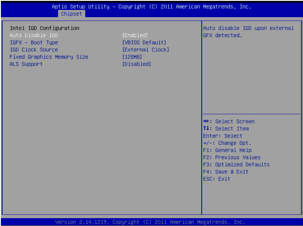
Figure 3.14 Chipset Setup
