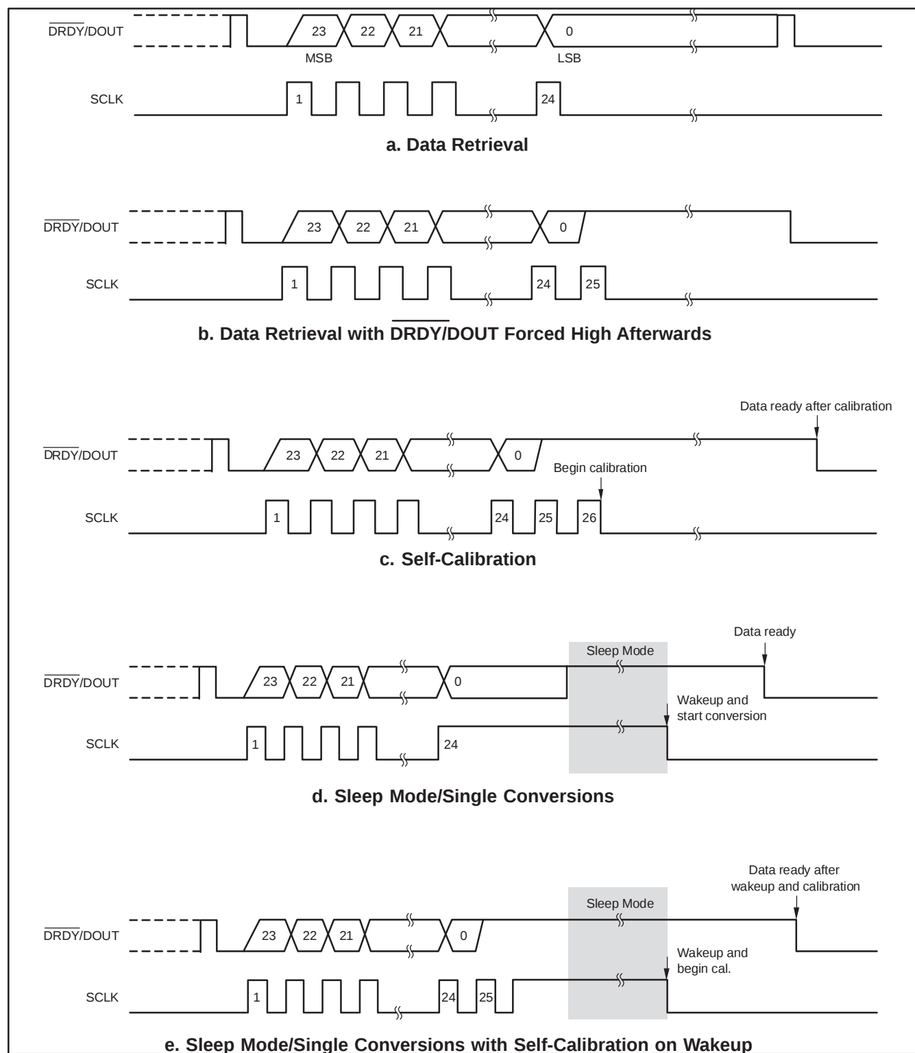
Figure 31. Summary of Serial Interface Waveforms
