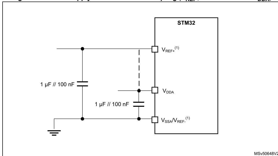
Figure 58. Power supply and reference decoupling ( V_{REF+} not connected to V_{DDA} )
