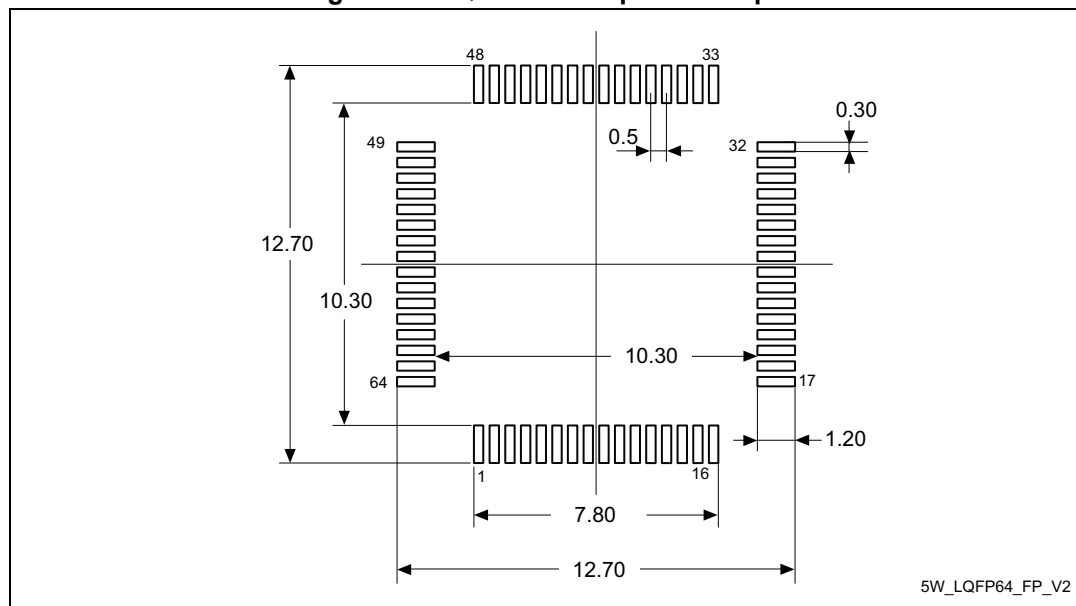
Figure 80. LQFP64 - Footprint example
