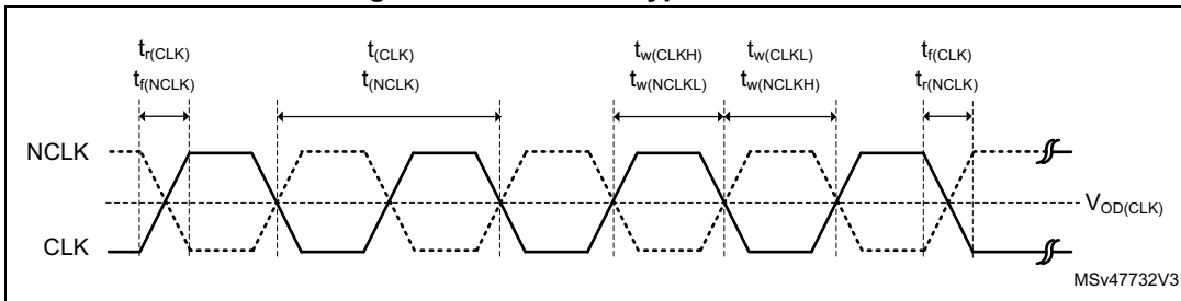
Figure 49. OCTOSPI hyperbus clock
