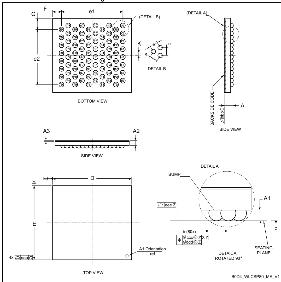
Figure 83. WLCSP80 - Outline
