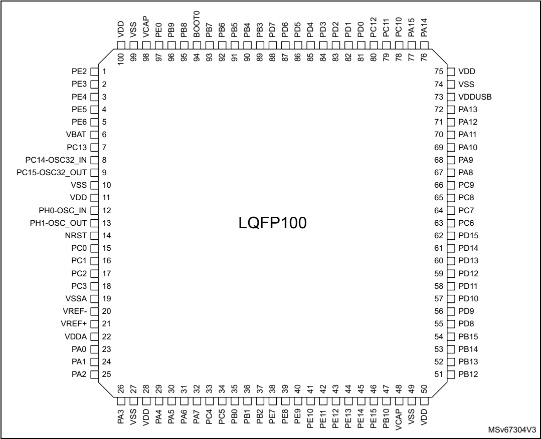
Figure 8. LQFP100 pinout
