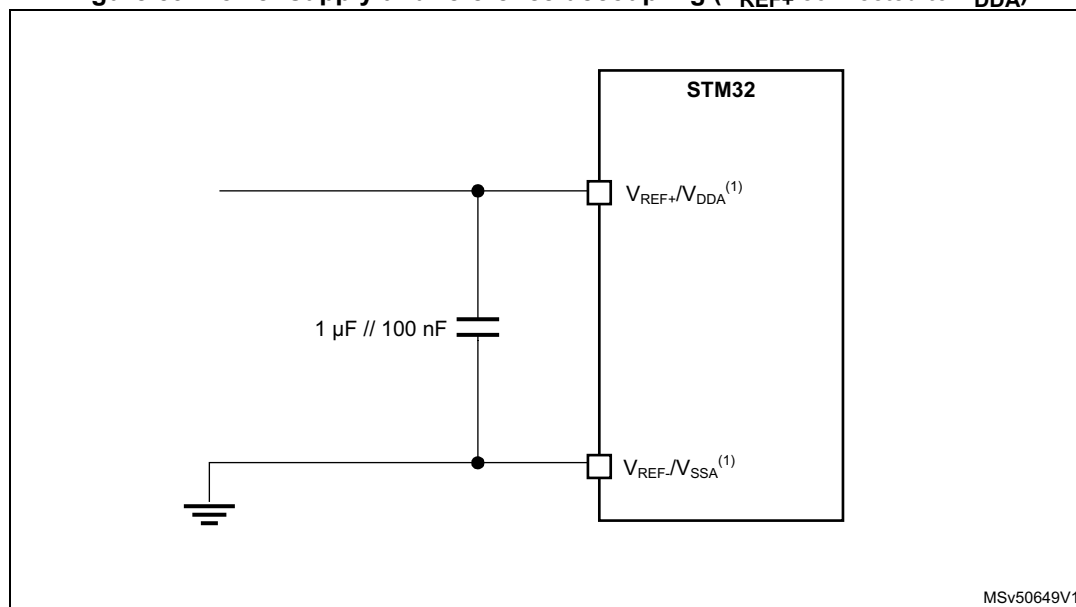
Figure 59. Power supply and reference decoupling ( V_{REF+} connected to V_{DDA} )
