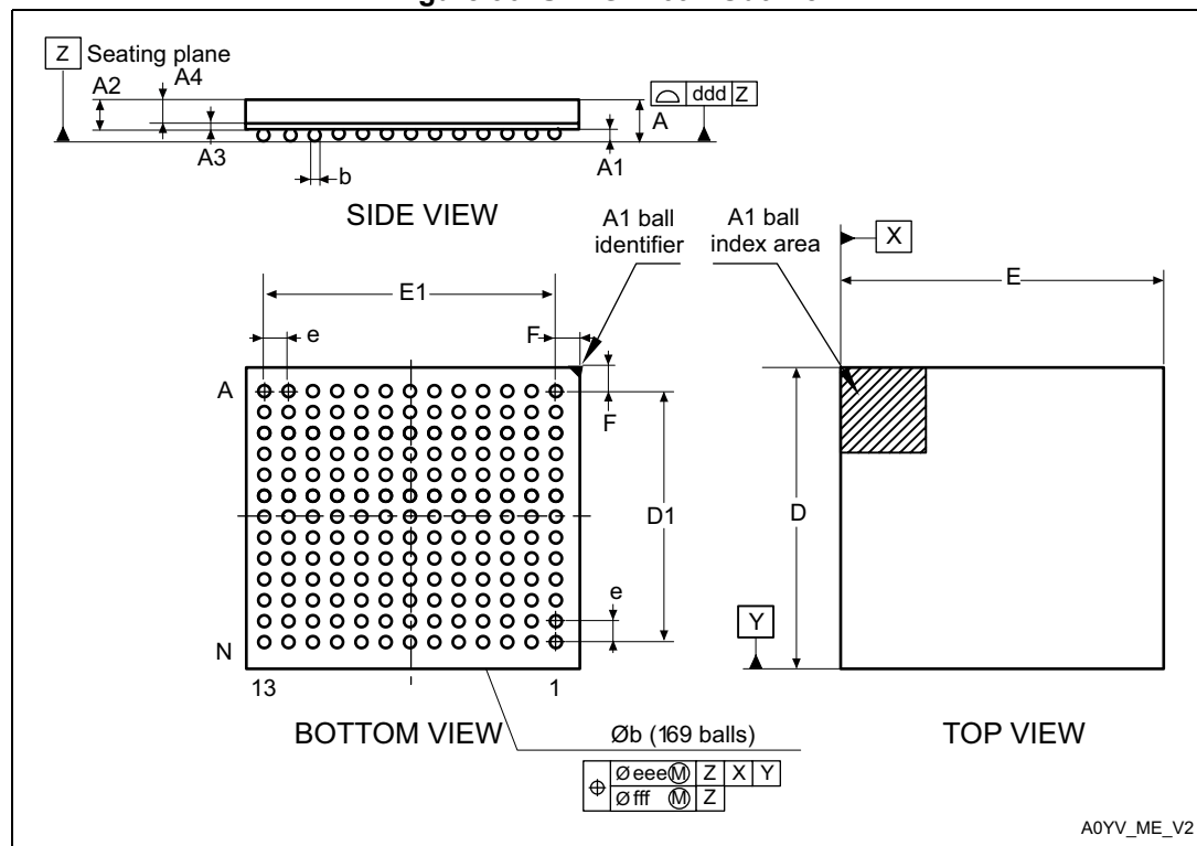
Figure 90. UFBGA169 - Outline
