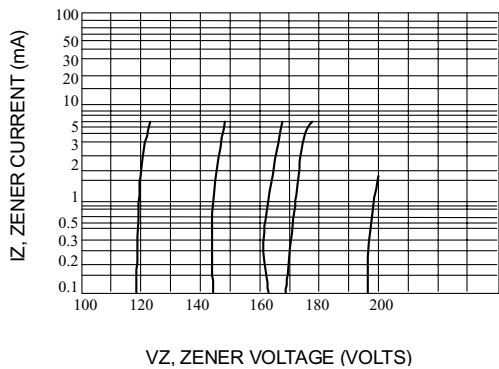
Fig. 8-VZ = 100 THRU 200 VOLTS
