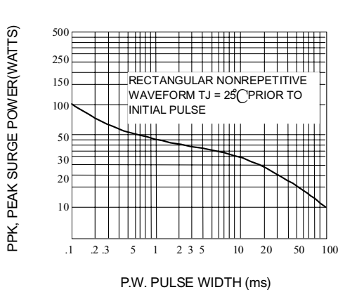
Fig. 2-MAXIMUM SURGE POWER
