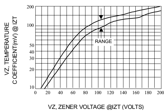
Fig. 5-UNITS 10 TO 200 VOLTS
