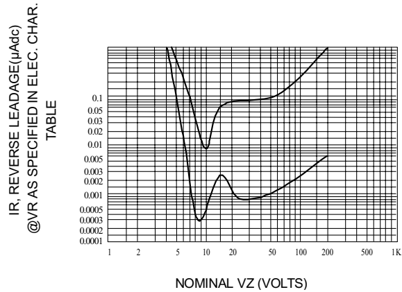
Fig. 3-TYPICAL REVERSE LEAKAGE
