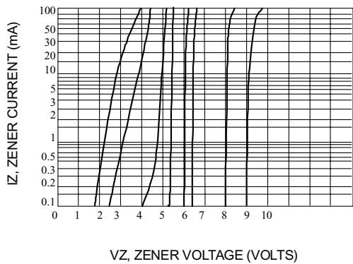
Fig. 6-VZ = 3.9 THRU 10 VOLTS
