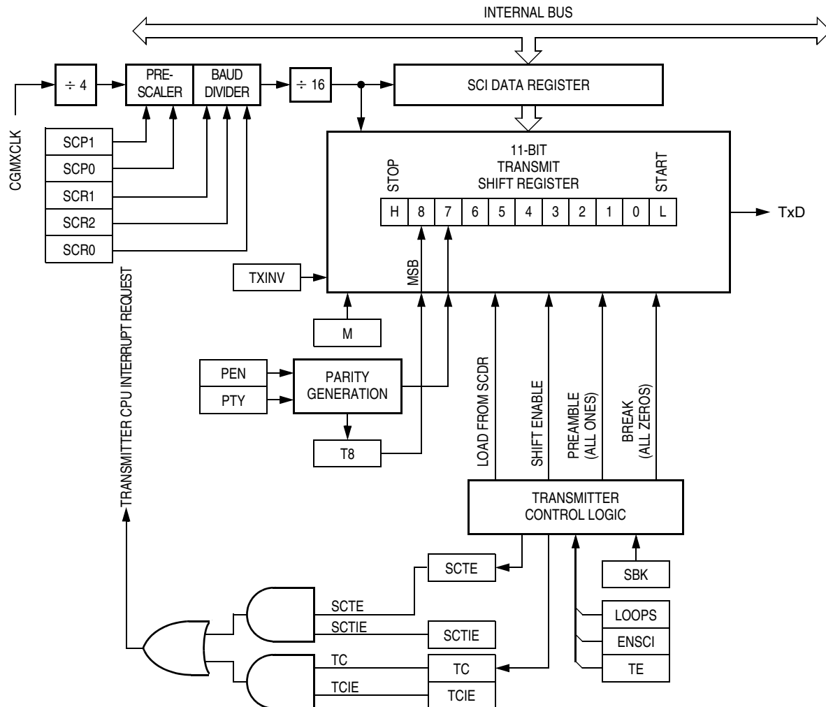
Figure 18-4. SCI Transmitter
