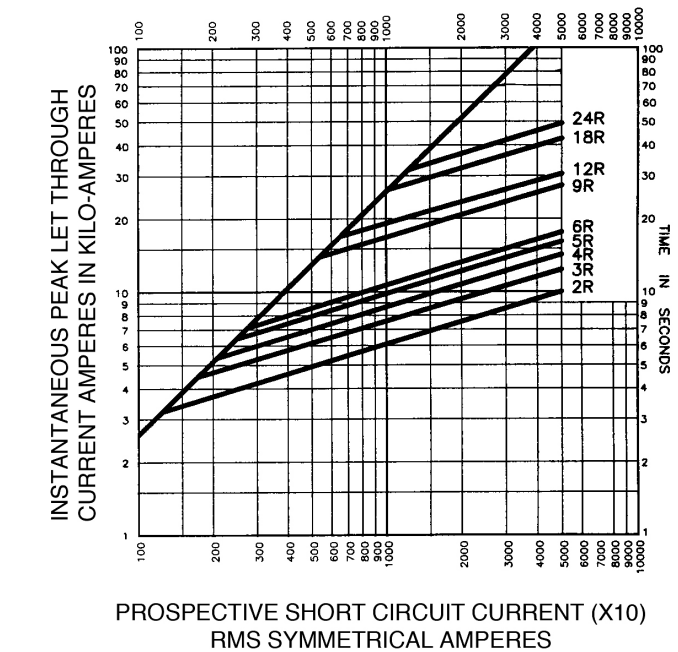
4.8 kV Peak let-through curves for JCL_R and JCL-A_R (2R-24R @25°C)
