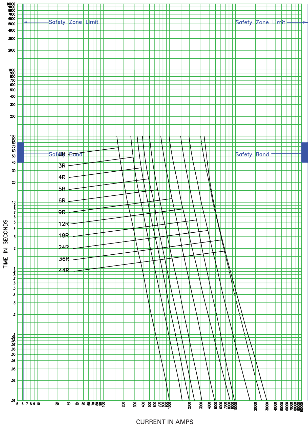
7.2 kV Time-current curves — minimum melting for 8CLS- R, 7CLS- R, 8ACLS- R, 7ACLS- R and 7BCLS- R (2R-44R @ 25C)
