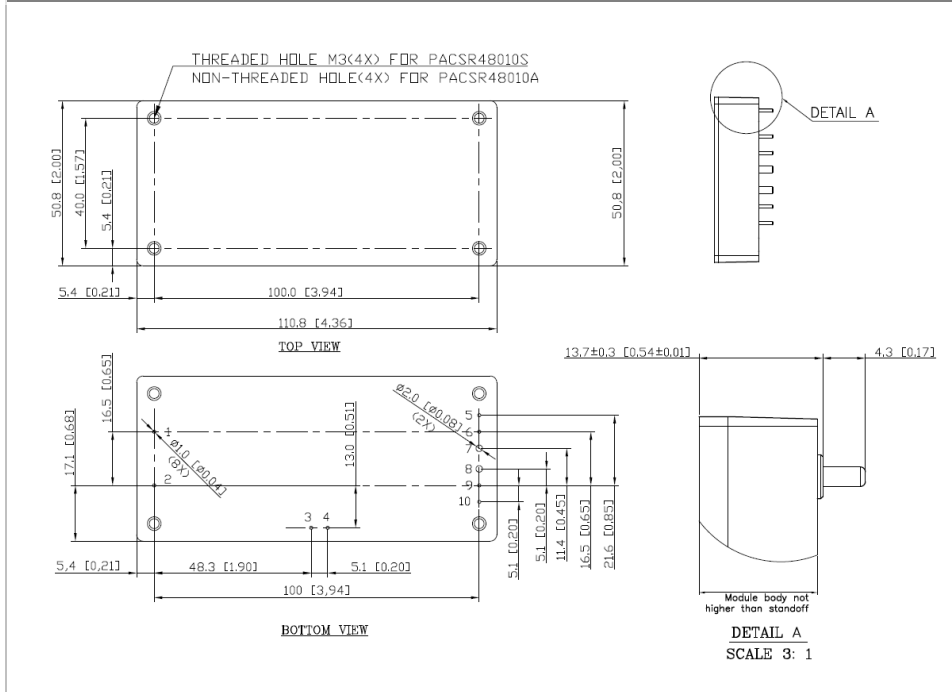
Mechanical Dimensions
