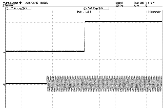
Figure 5: Vout start up with Enable on at 220Vac, 10.5A Iout, TOP: Vout, 20V/div, 500ms/div
