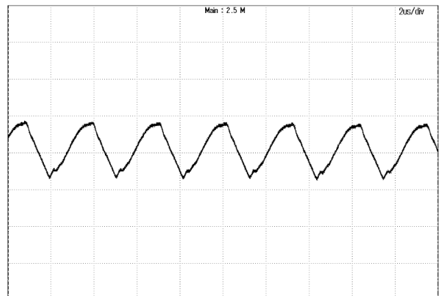
Figure 10: Output Voltage Ripple and Noise at nominal input voltage and max load current (100mV/div, 2us/div) Load cap: 470µF Oscon cap. Bandwidth: 20MHz.
