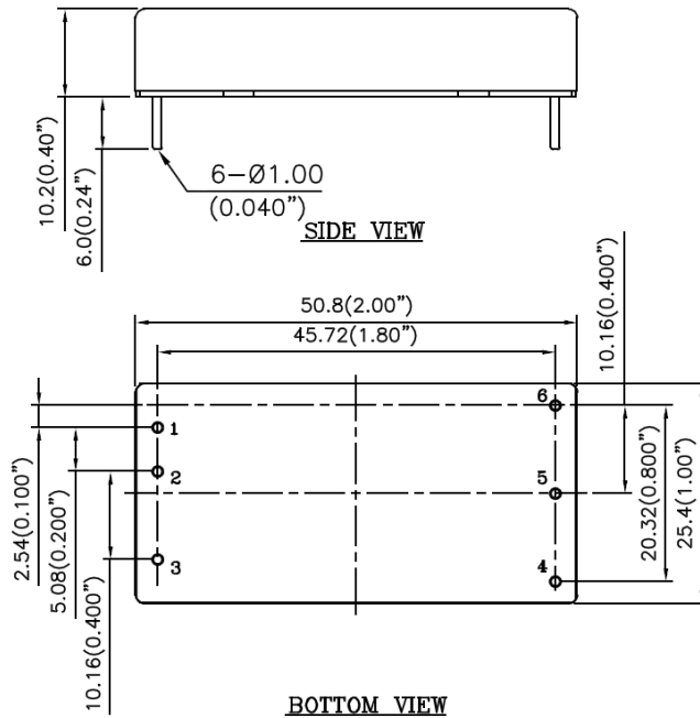
Mechanical Dimensions
