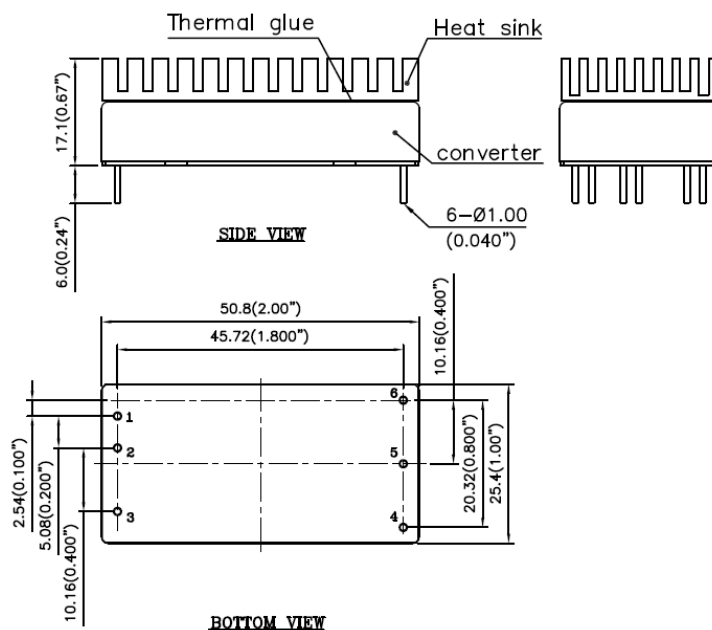
Mechanical Dimensions
