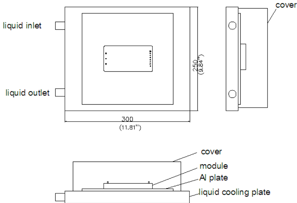
Figure 10: Thermal test setup
