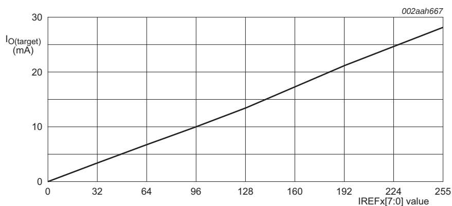
Fig 12. I_{\text{O(target)}} versus IREFx value with R_{\text{ext}} = 2 \text{ k}\Omega
