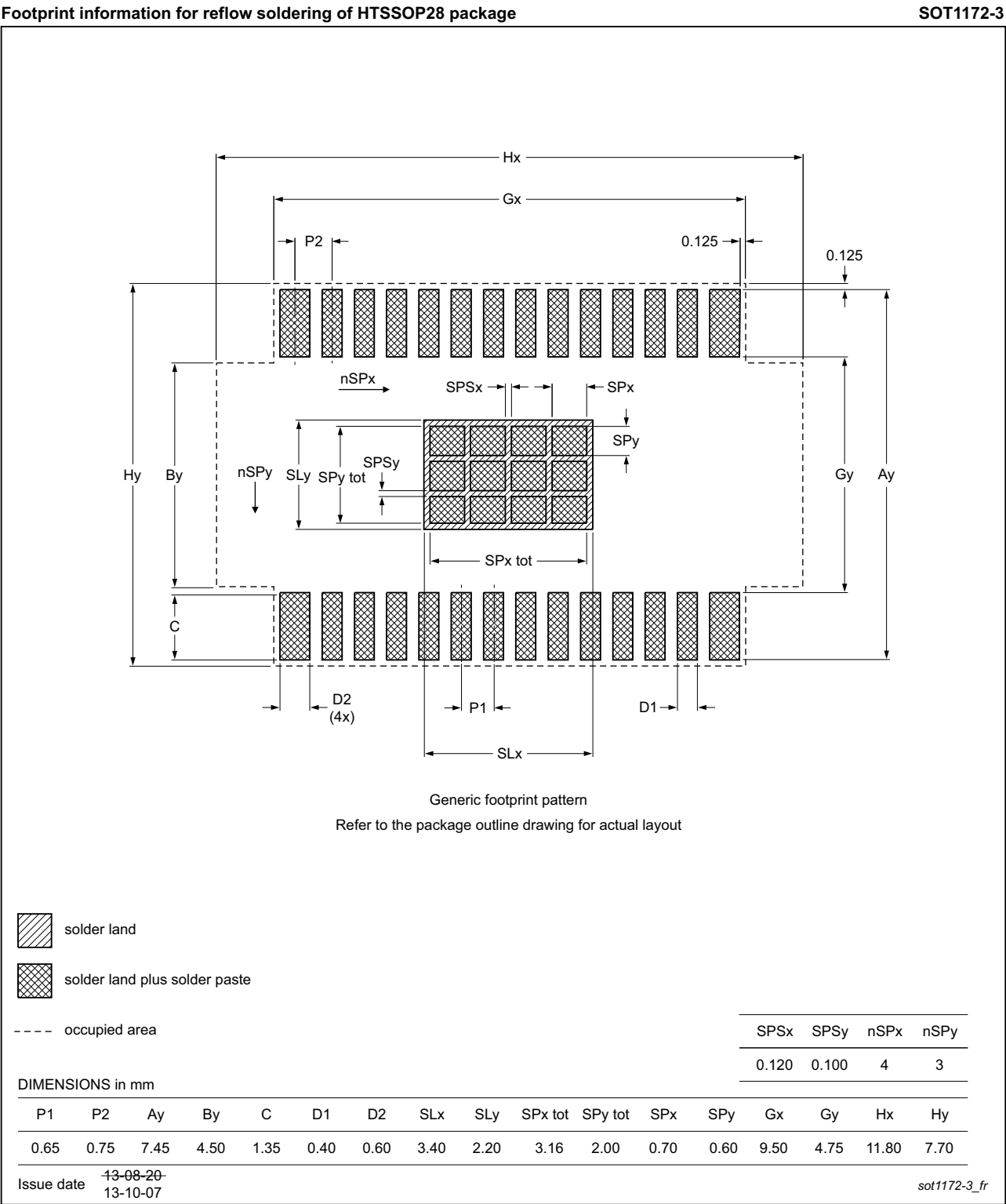
Fig 31. PCB footprint for SOT1172-3 (HTSSOP28); reflow soldering
