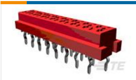
TE Part #215079-8 MICRO-MATCH FOB.08P
