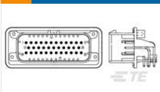
TE Part #1-776180-1 35POS,PIN DIA 1.3,HDR ASSY,90DEG, COD 1
