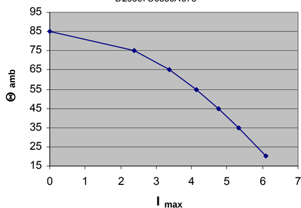
Max. allowable ambient Temp. at specific current (rms) B25667C6336A375
