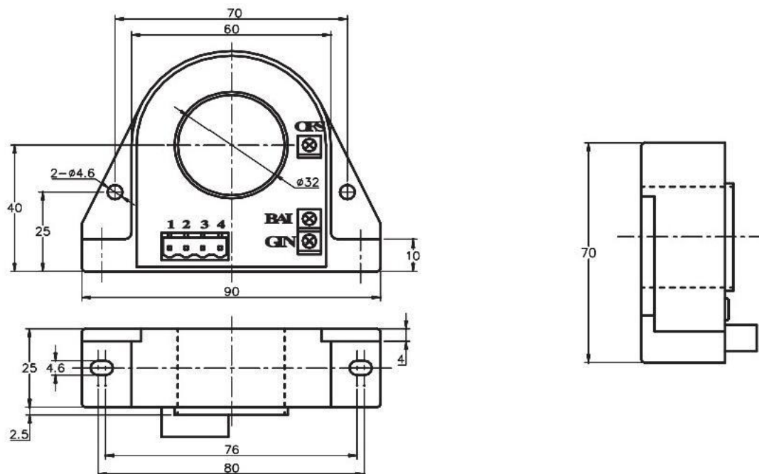
外形尺寸(mm)/Dimensions of drawing(mm)
