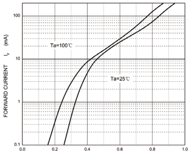
Forward Characteristics
