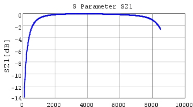
GRM1885C1H3R3WA01 S21 DCOV, 25degC
