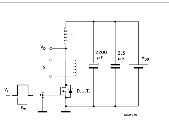
Figure 19. Unclamped inductive load test circuit
