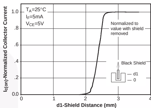
Figure 2. Normalized Collector Current Vs. Shield Distance
