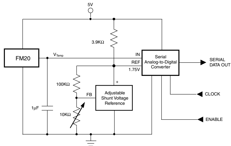
Figure 4. Serial Output Temperature to Digital Converter
