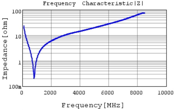
GCH1885C2A680JE01 |Z| DCOV, 25degC
