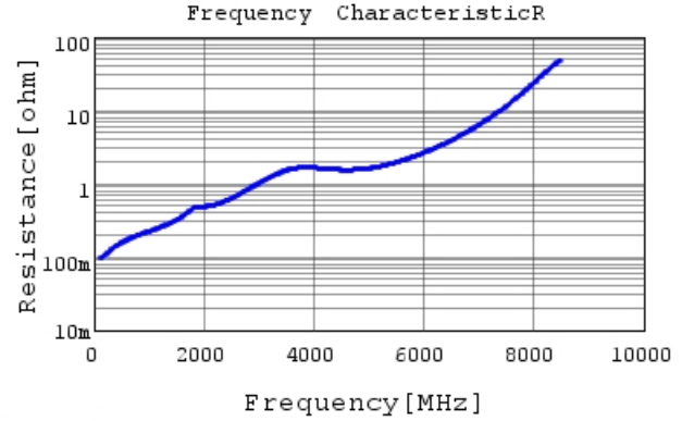
GCH1885C2A680JE01 R DCOV, 25degC
