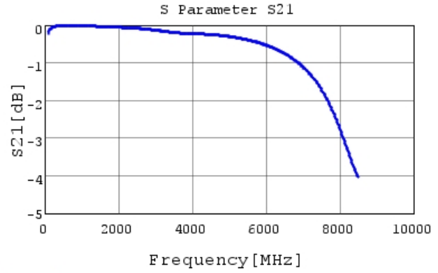
GCH1885C2A680JE01 S21 DCOV, 25degC
