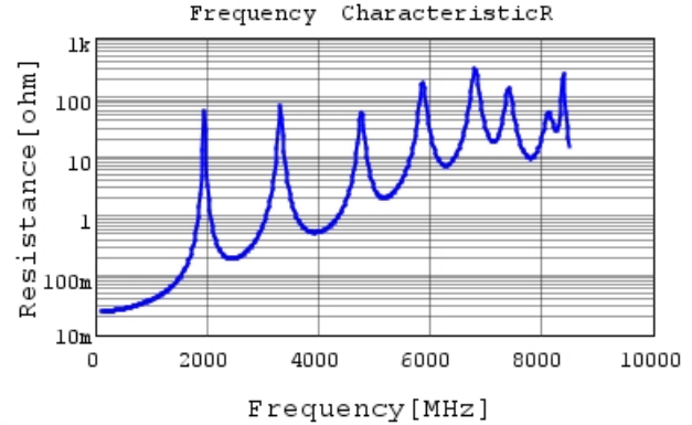
GQM22M5C2H680JB01 R DCOV, 25degC
