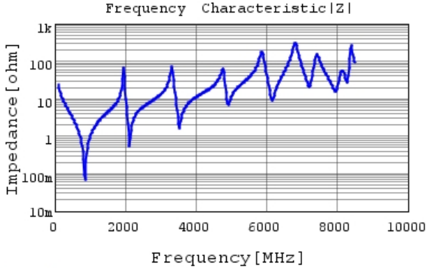
GQM22M5C2H680JB01 |Z| DCOV, 25degC
