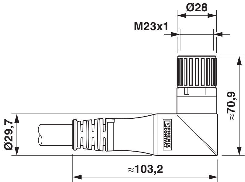
Dimensional drawing
